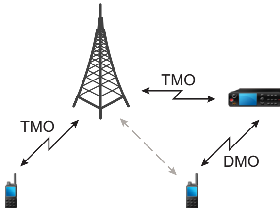
Figure 10: Gateway Mode Operation
