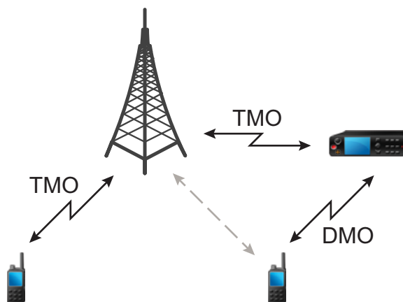
Figure 12: Communication through Gateways
