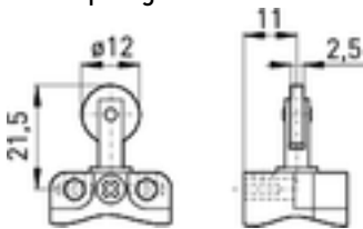
Roller plunger R
