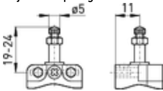
Adjustable plunger ST
