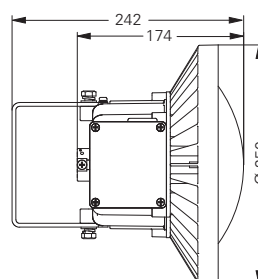
Dimension drawing LEL Portable 5L
